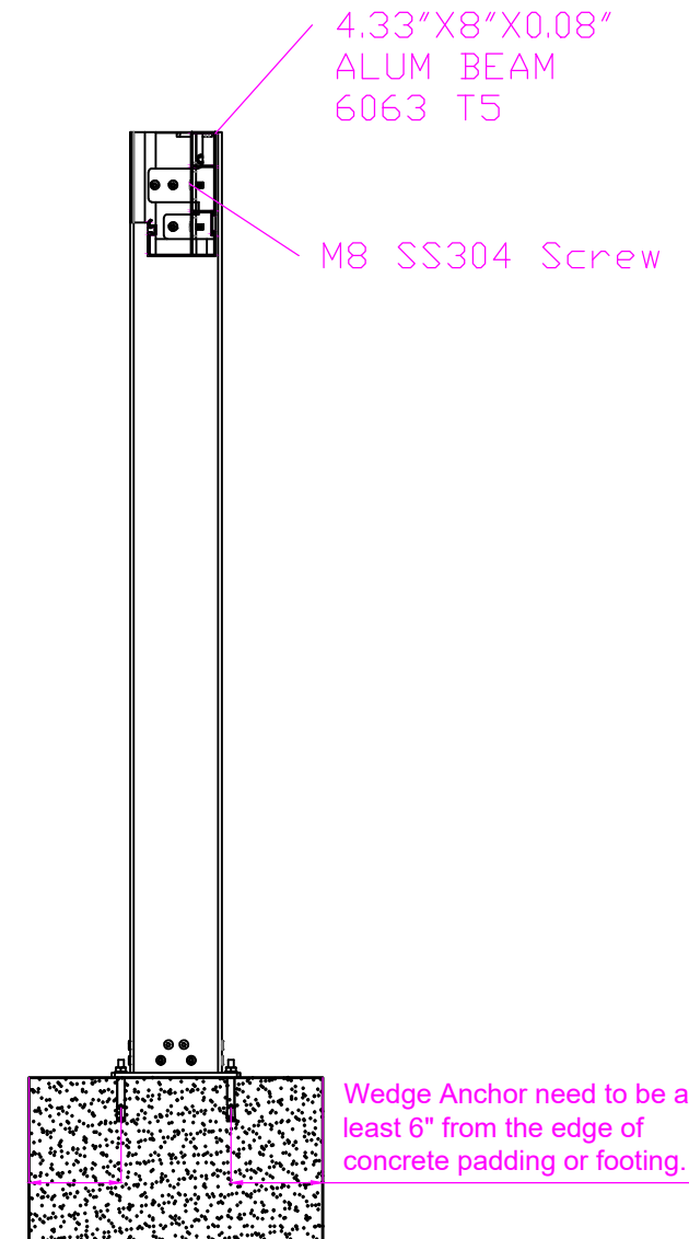
SECTION A-A LOUVER BEAM REINF. DETAIL
