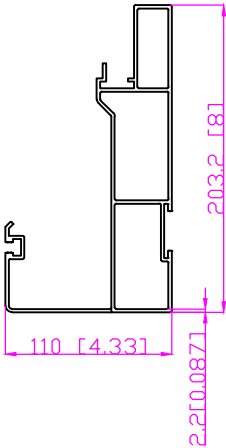
Louver Beam
