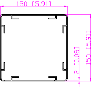
Column
