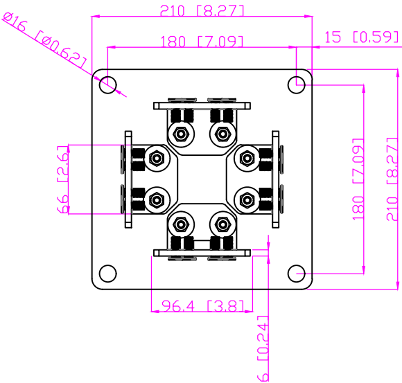
Footing Plate
