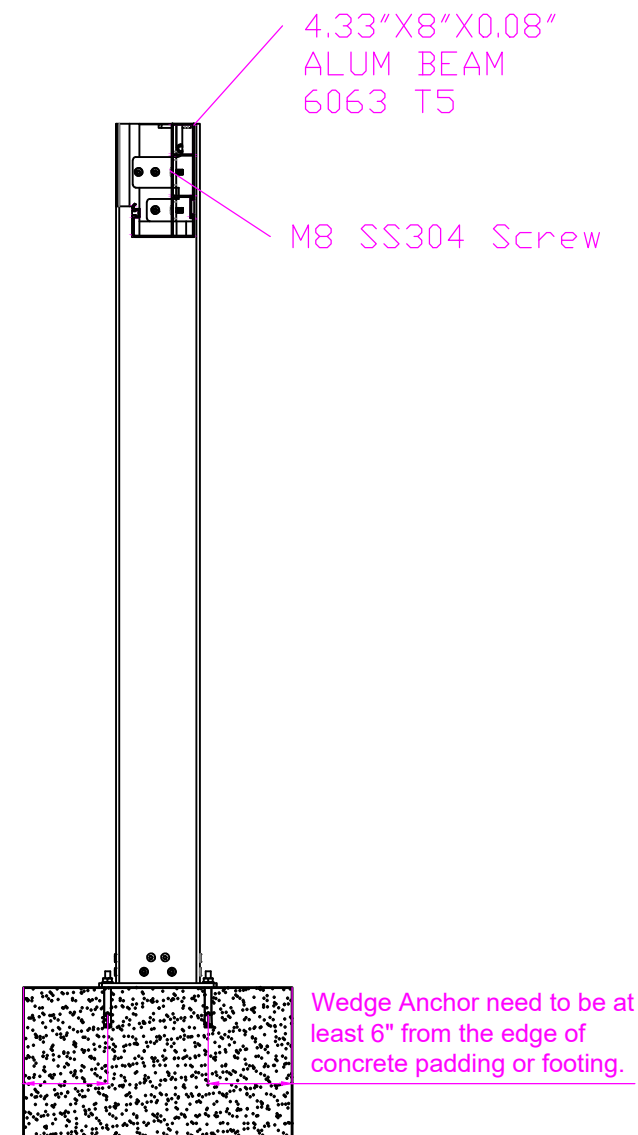
SECTION A-A LOUVER BEAM REINF. DETAIL
