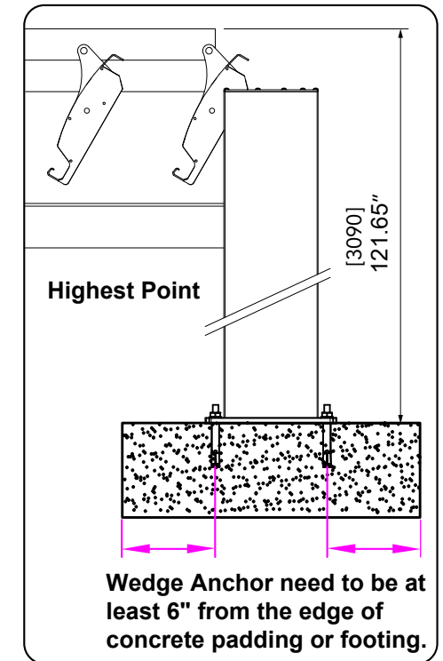
DETAIL-A
