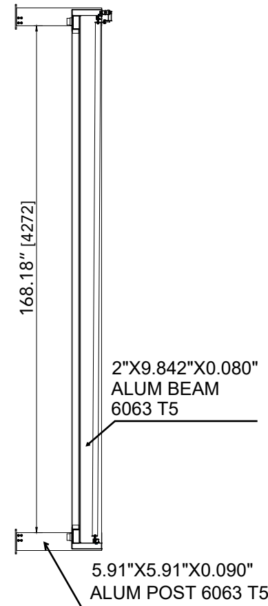
LATERAL VIEW 1
