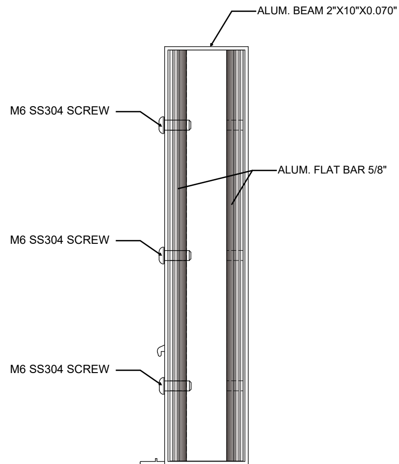
SECTION A-A LOUVER BEAM REINF. DETAIL
