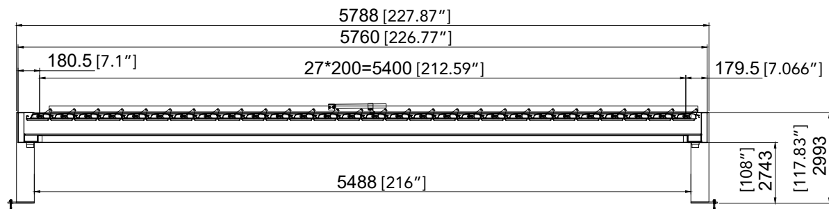
TOP VIEW
