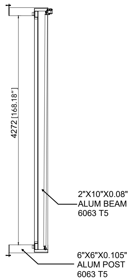
LATERAL VIEW 1
