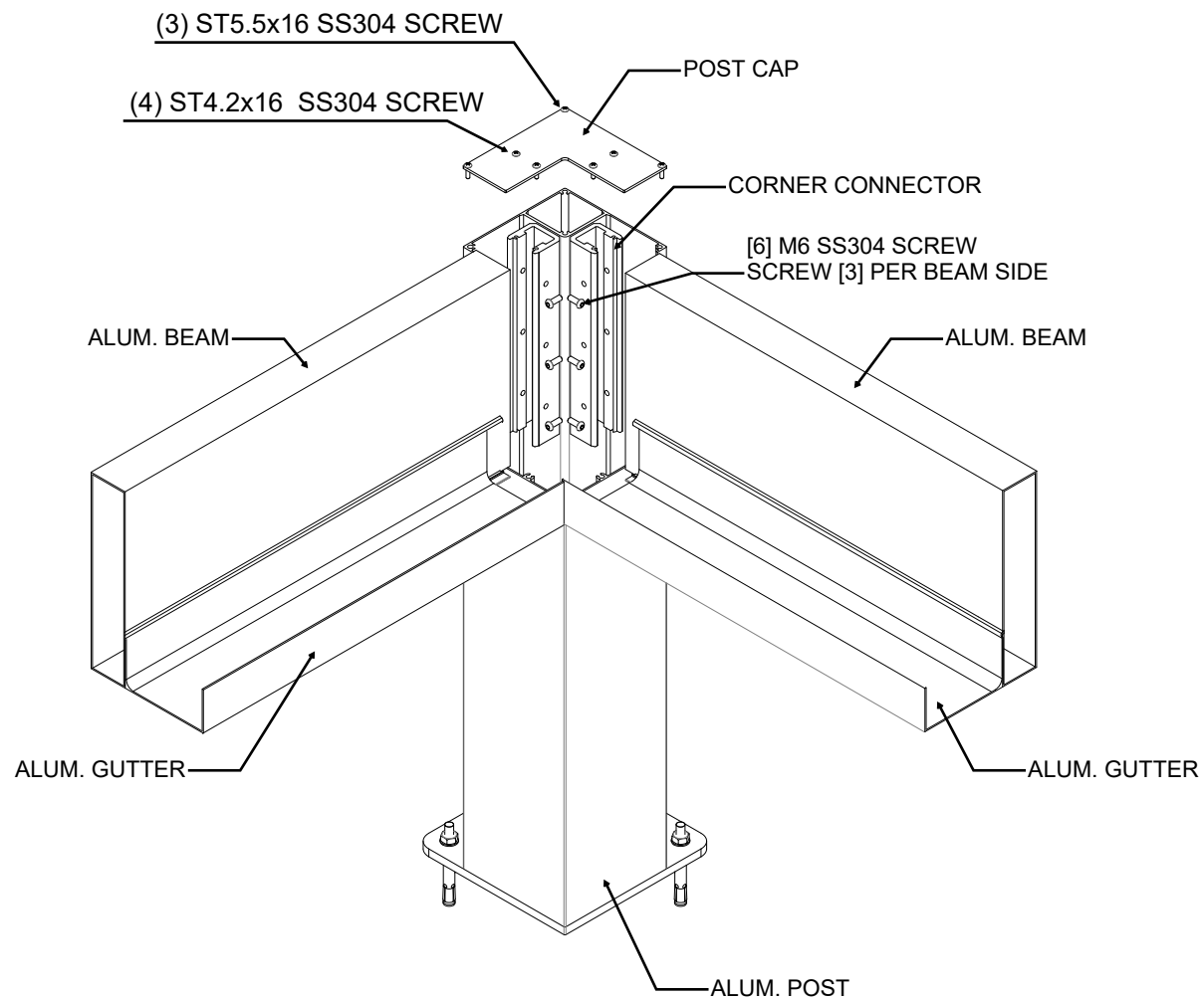
BEAM-POST CONNECTION
