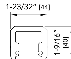
CORNER CONNECTOR
