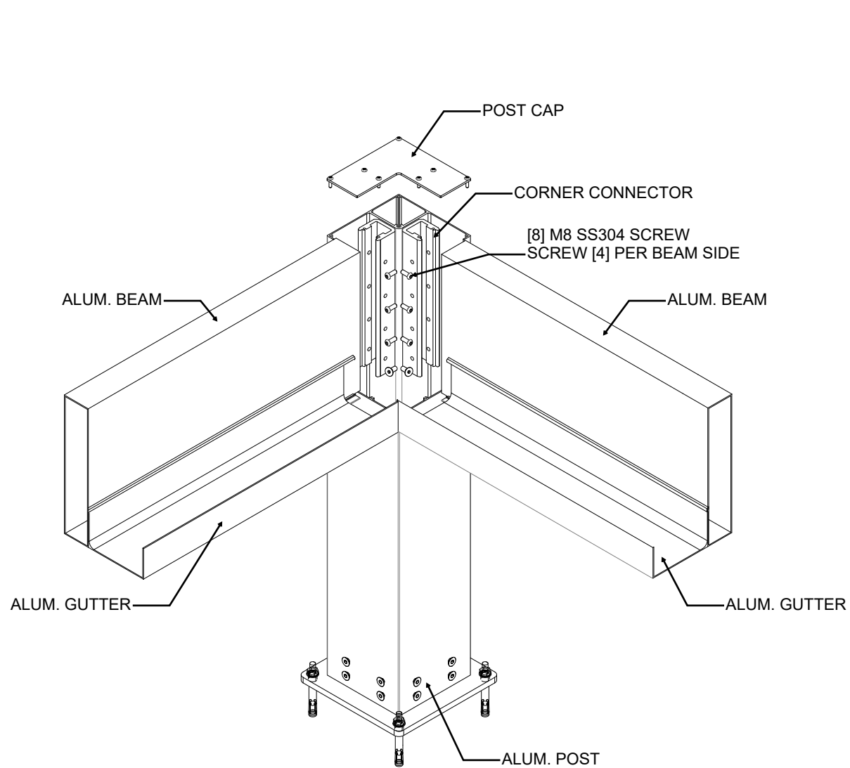
BEAM-POST CONNECTION
