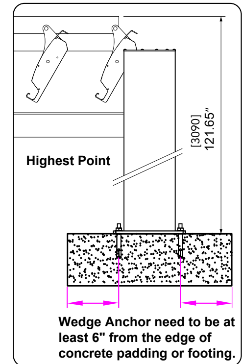
DETAIL-C
